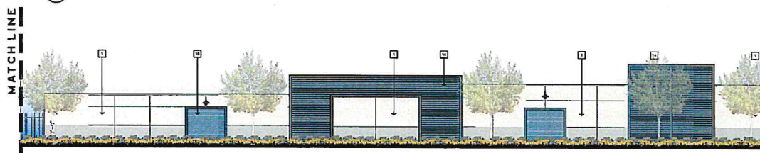
1B ENLARGED NORTH ELEVATION - SIERRA STREET (CONT.)
