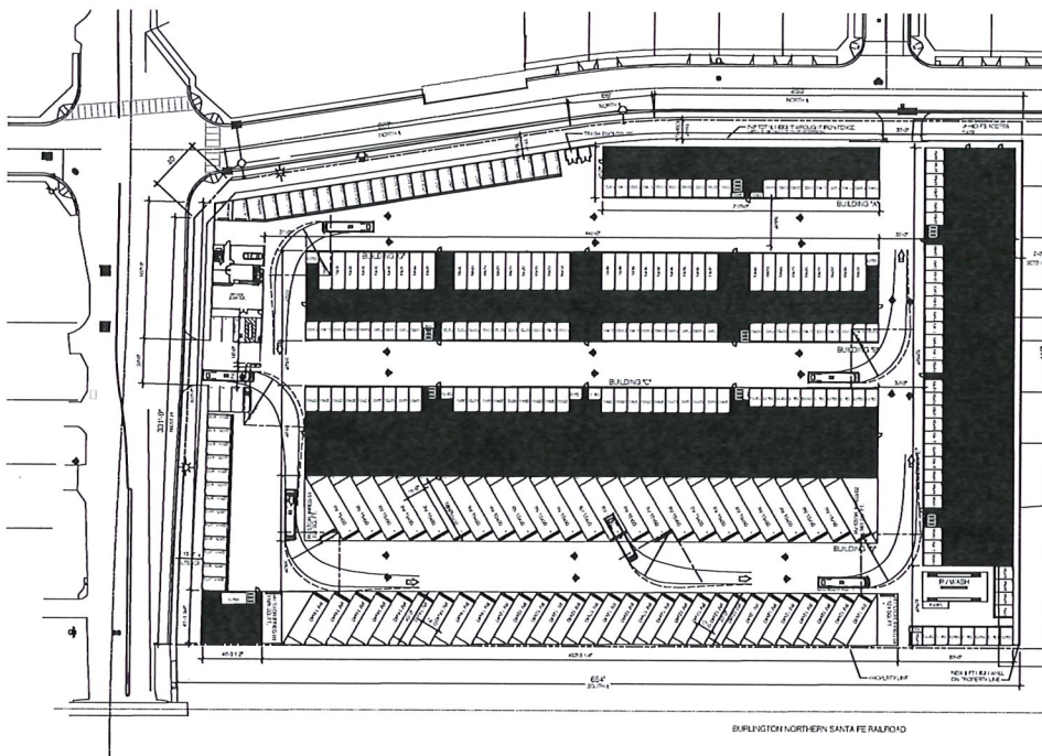
1 PROPOSED SITE PLAN 1/32\"/>
