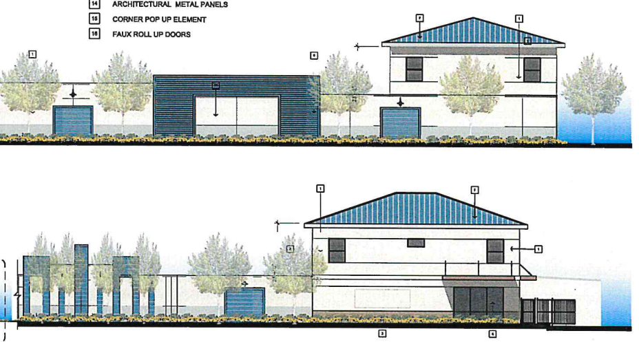
2A ENLARGED WEST ELEVATION
