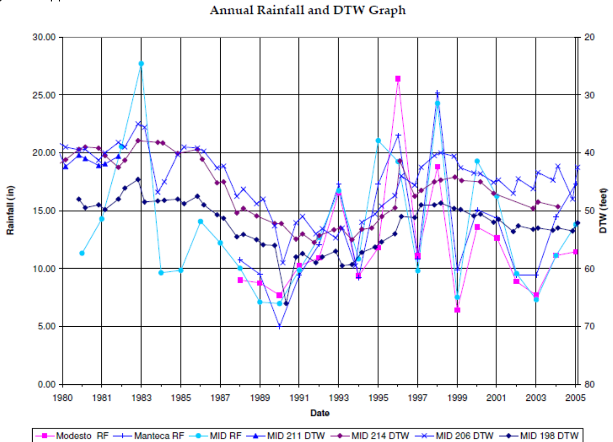
Figure 4.4 - Comparison of average rainfall (RF) and depth to groundwater in Modesto Irrigation District monitoring wells (MID).
